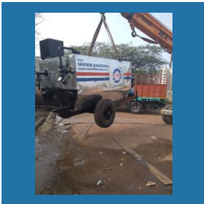
Bitumen Emulsion Sprayer
