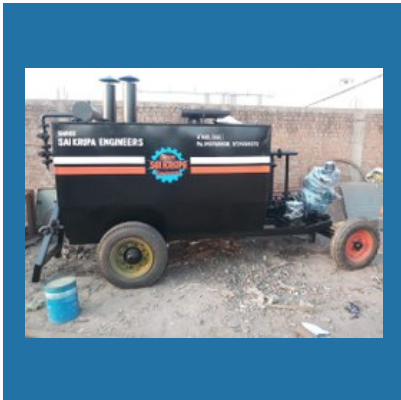
Tar Boilers
